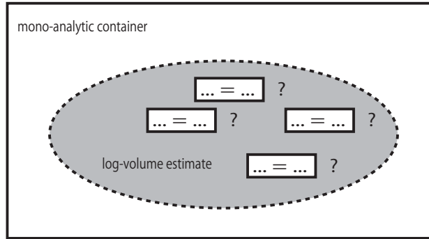
Fig. 1.1: Log-volume estimate region inside a mono-analytic container
