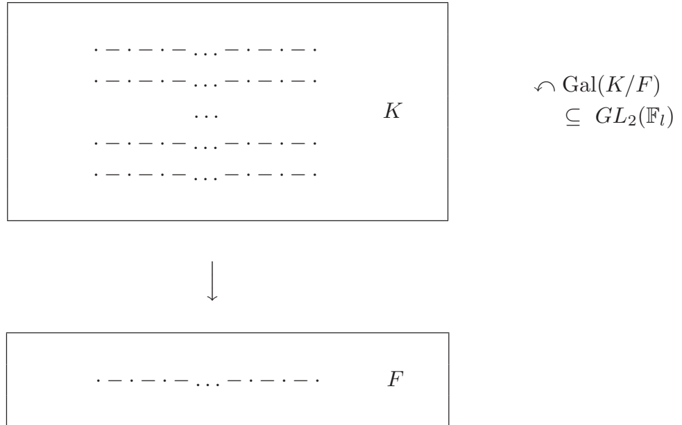
Fig. 3.2: Prime-strips as “sections” of \mathrm{Spec}(K) \rightarrow \mathrm{Spec}(F)
