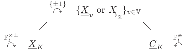
Fig. 3.3: Symmetries of coverings of X_F
