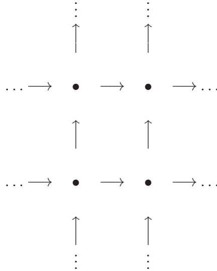
Fig. 3.1: The log-theta-lattice consists of “ \bullet ” [i.e., \Theta^{\pm\text{ell}} NF-Hodge theaters ], “ \uparrow ” [i.e., log-links ], and “ \rightarrow ” [i.e., \Theta -links]
