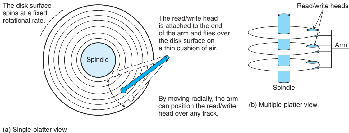
Figure 6.10 Disk dynamics.
