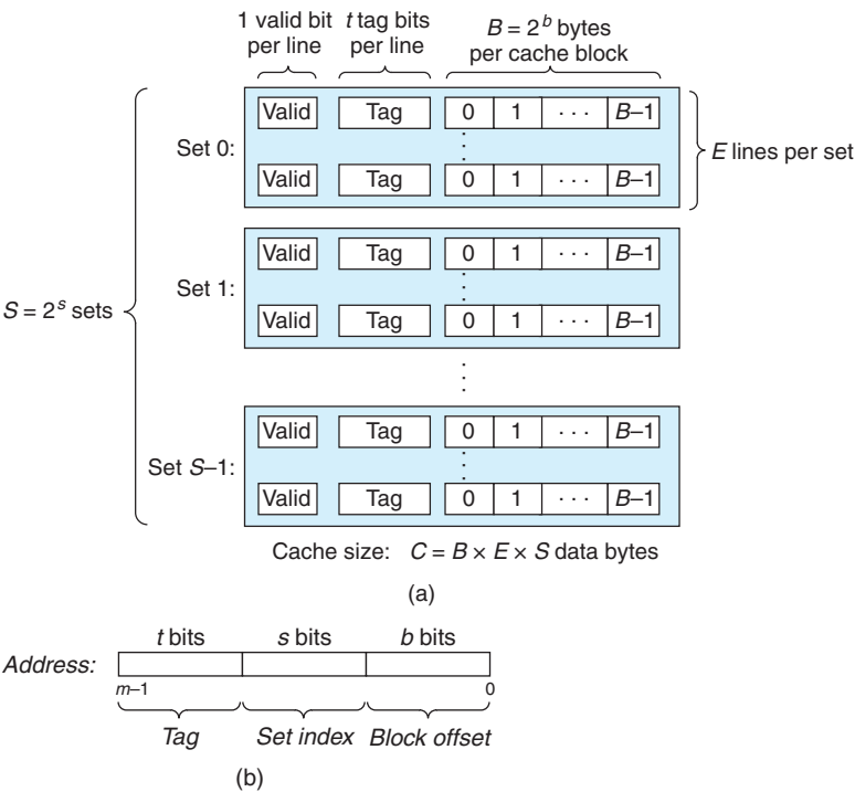
Figure 6.25 General organization of cache ( S, E, B, m ). (a) A cache is an array of sets. Each set contains one or more lines. Each line contains a valid bit, some tag bits, and a block of data. (b) The cache organization induces a partition of the m address bits into t tag bits, s set index bits, and b block offset bits.
