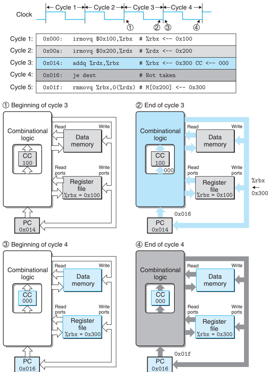
Figure 4.25 Tracing two cycles of execution by SEQ. Each cycle begins with the state elements (program counter, condition register, register file, and data memory) set according to the previous instruction. Signals propagate through the combinational logic, creating new values for the state elements. These values are loaded into the state elements to start the next cycle.
