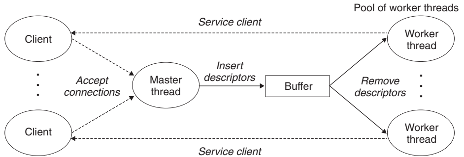
Figure 12.27 Organization of a prethreaded concurrent server. A set of existing threads repeatedly remove and process connected descriptors from a bounded buffer.
