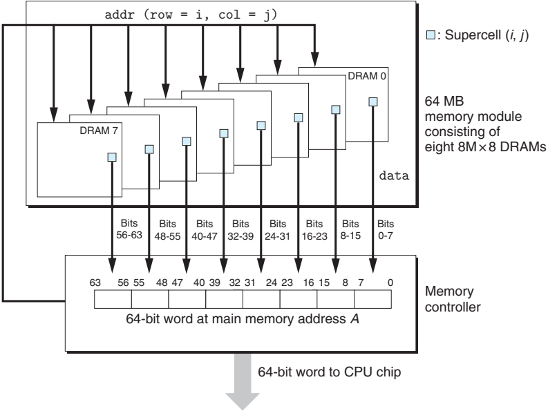
Figure 6.5 Reading the contents of a memory module.
