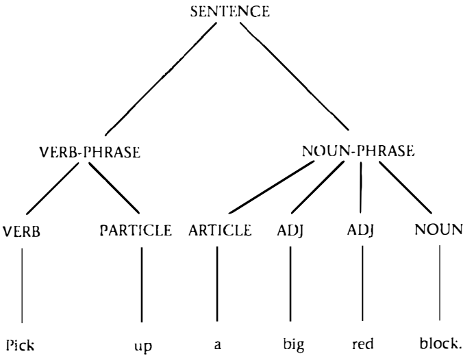
Figure 10.1 A "tree" representation of the sentence "Pick up a big red block."
