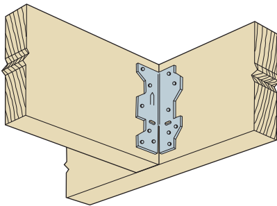
A35-type 3 Angle
