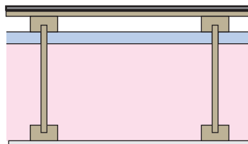
Vented cathedral ceiling with I-joint rafters
