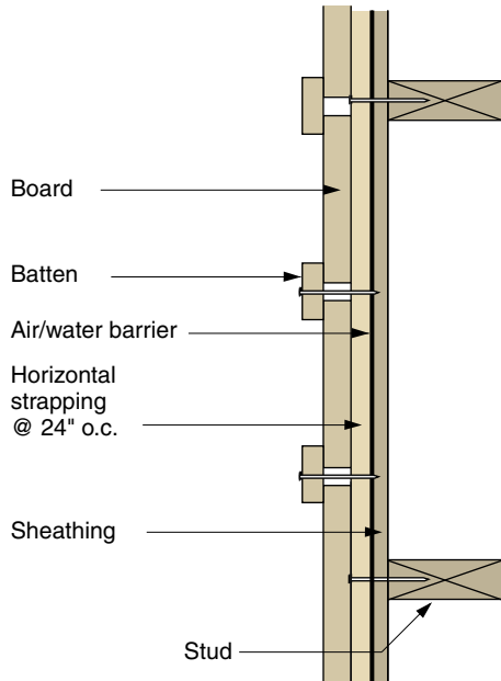
BOARD & BATTEN
