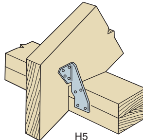
H5 Hurricane Tie
