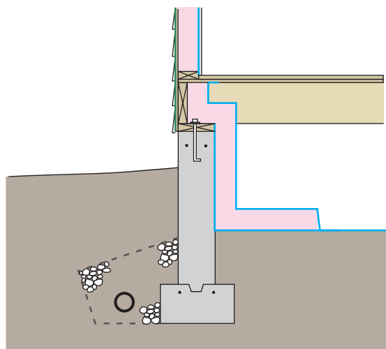
Unvented crawl space with interior batt perimeter insulation
