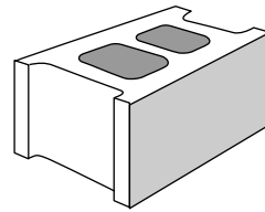
Stretcher 11 5 / 8 "x15 5 / 8 "x7 5 / 8 "
