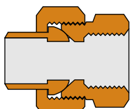
Union, Copper to Fnpt
