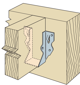
U Hanger
