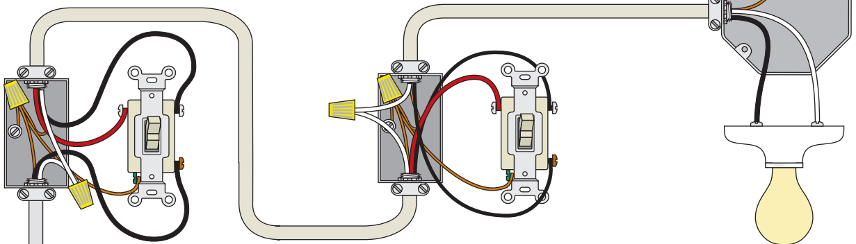
LIGHT AT END OF 3-WAY SWITCHES
