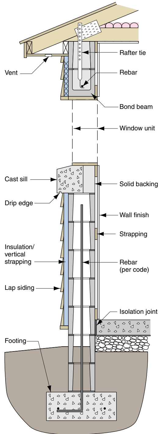
WITH HORIZONTAL LAP SIDING
