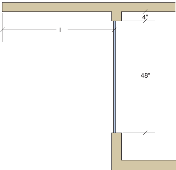
Overhang Geometry for Table
