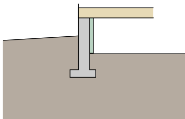
Unvented concrete with rigid interior insulation
