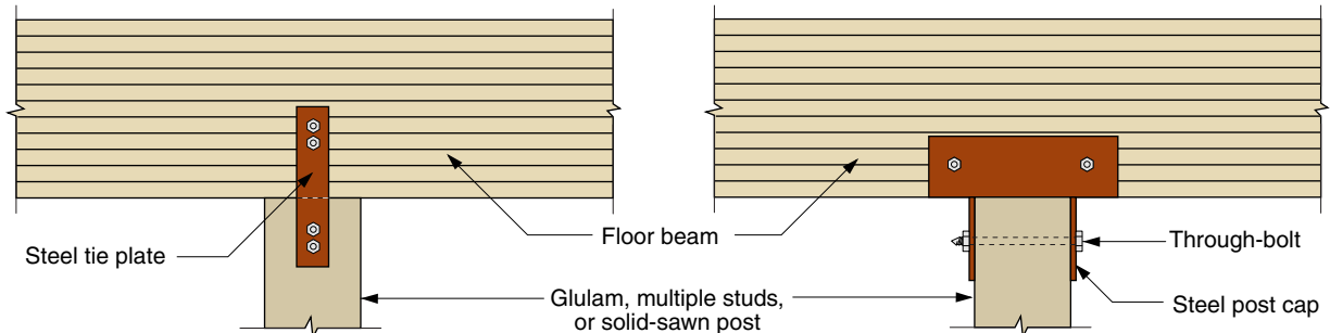
CONTINUOUS FLOOR BEAM OVER INTERMEDIATE WOOD SUPPORTS
