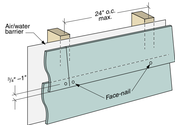
FASTENING OPTION 2
