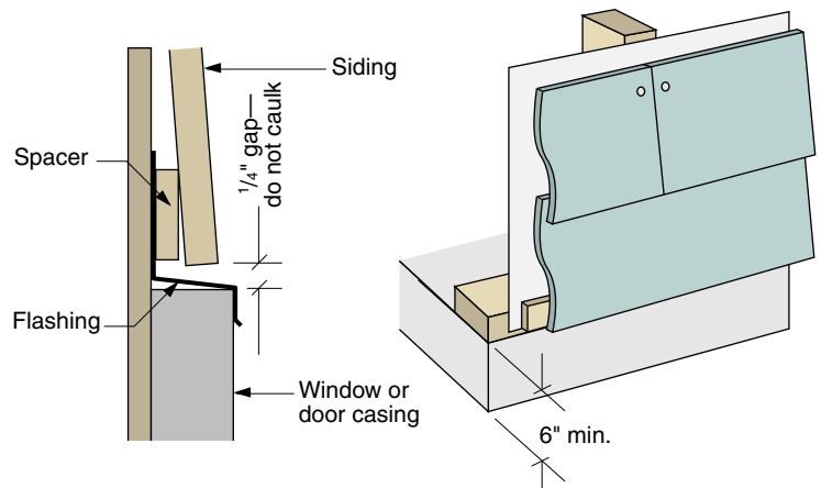
FASTENING OPTION 2
