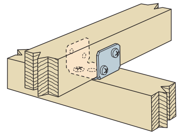
RTU2 Rigid Tie
