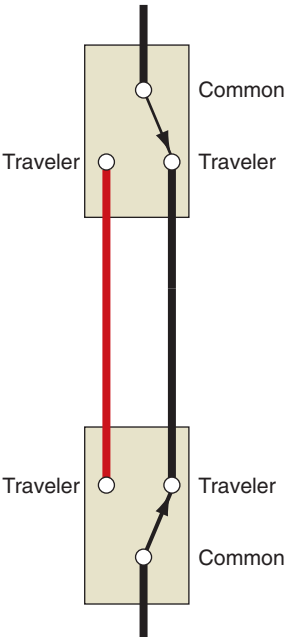
3-WAY SWITCH (used in pairs)
