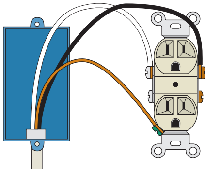
PLASTIC BOX, END OF CIRCUIT
