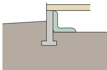
Unvented concrete with blanket interior insulation
