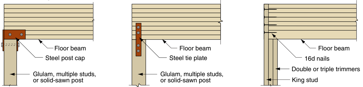
BEAM BEARING AT END WALL
