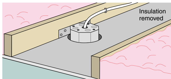
BEFORE SEALING
