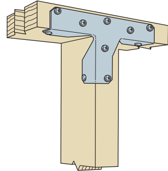
RTT22 Rigid Tie
