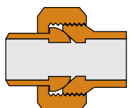
Union, Copper to Copper
