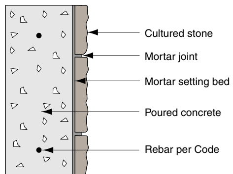
OVER POURED CONCRETE
