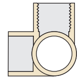
Side Outlet Ell, Slip x Slip x Fipt
