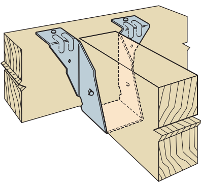
PF Hanger
