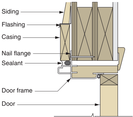
HEAD
