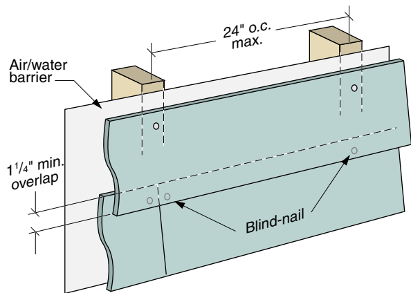
FASTENING OPTION 1
