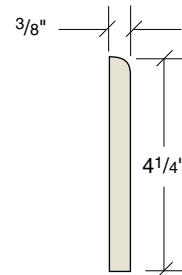
4 1/4" x 4 1/4" surface bullnose
