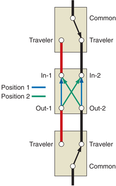
4-WAY SWITCH (used between pair of 3-ways)
