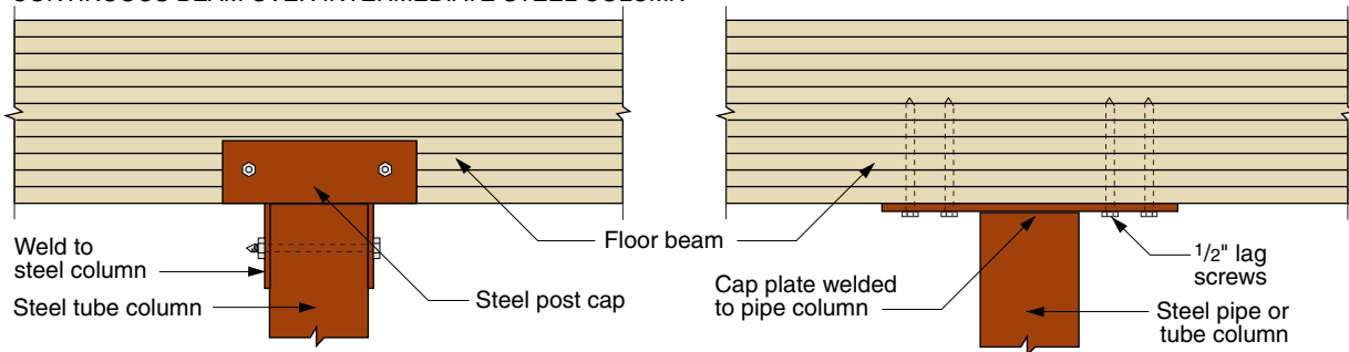
CONTINUOUS BEAM OVER INTERMEDIATE STEEL COLUMN
