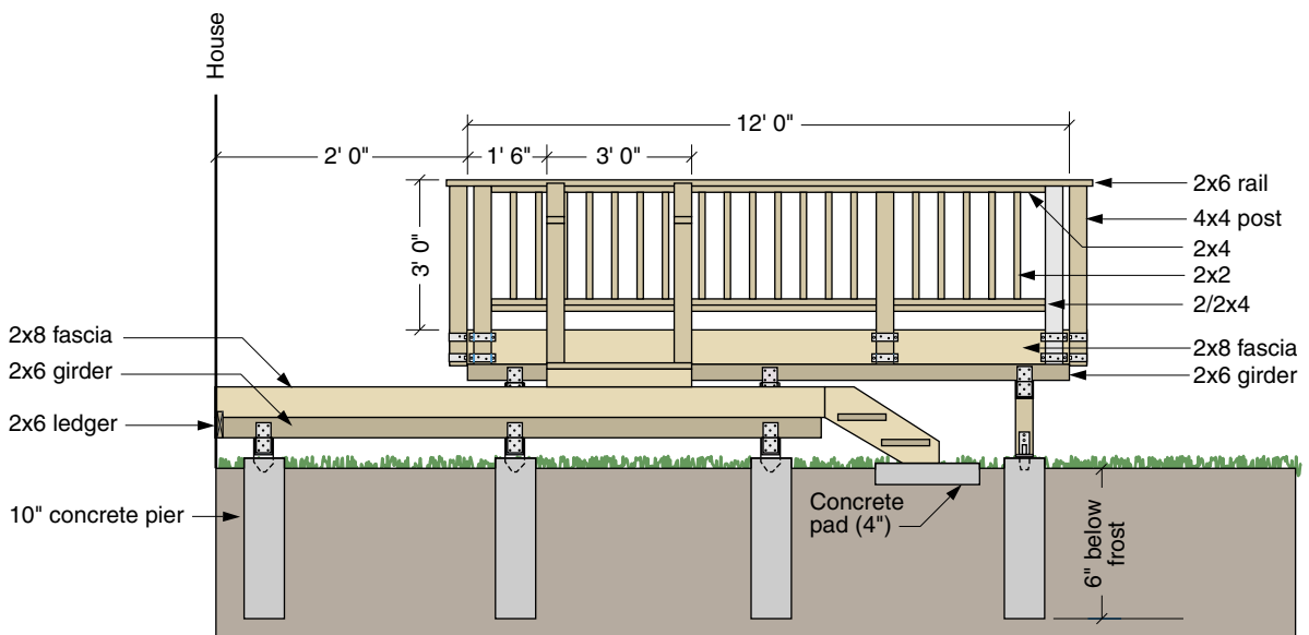
LEFT ELEVATION
