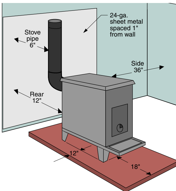
Radiant Stove with Rear Protection
