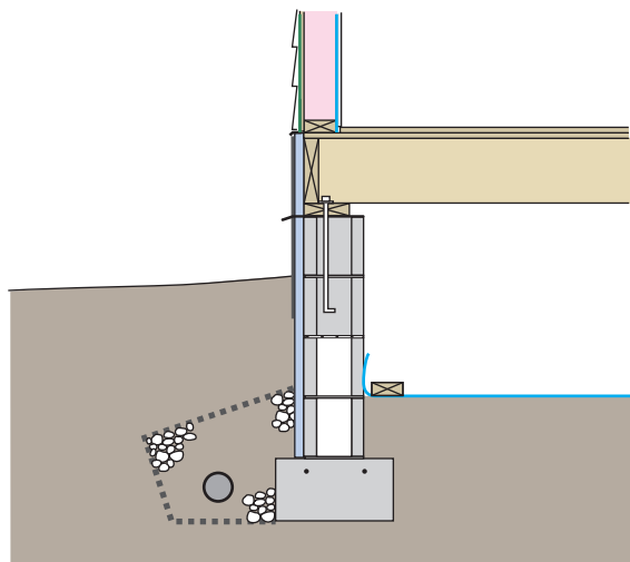
Unvented crawl space with exterior foam perimeter insulation
