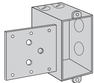
Box with side bracket
