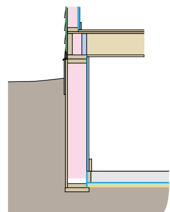
All-weather wood foundation with batt insulation
