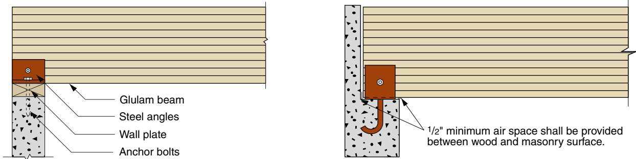
BEAM BEARING AT MASONRY WALL
