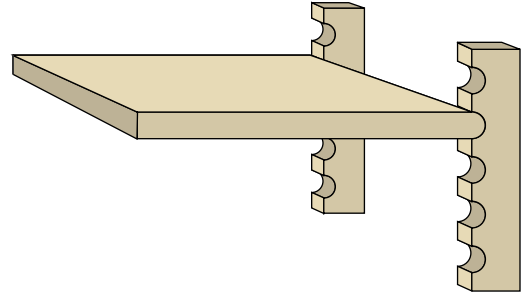
SPLIT 2X4 WITH \frac{7}{8} " HOLES
