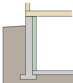
Concrete wall with full-height interior insulation
