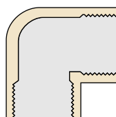
90 El, Fipt x Fipt
