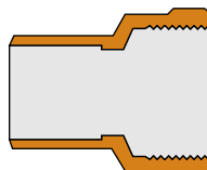
Reducing Female Adaptor, Copper to Fnpt
