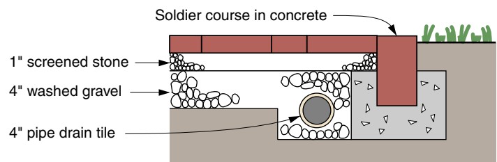
PATIO-GRAVEL BASE
