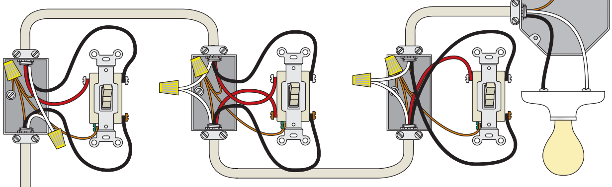
4-WAY SWITCH
