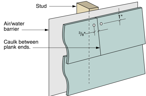
JOINT OPTION 2
