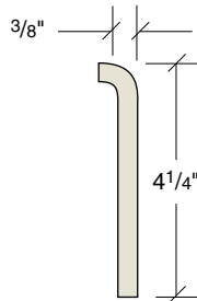
4 1/4" x 4 1/4" bullnose
