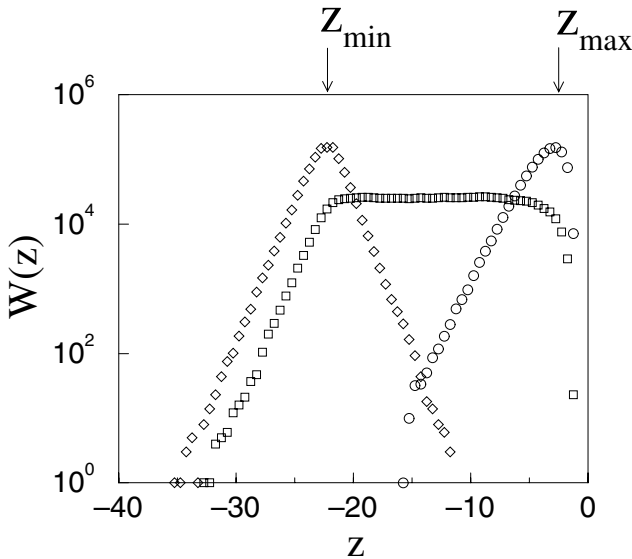
Figure 13.5. The exponential distributions of the variable z (corresponding to the power-law distributions of w ) for coupled skew tent maps as in Fig. 13.3, for three values of coupling: critical coupling \varepsilon = \varepsilon_c (squares); coupling larger than critical \varepsilon = \varepsilon_c + 0.025 (diamonds); coupling smaller than critical \varepsilon = \varepsilon_c - 0.025 (circles). An additional parameter mismatch a \pm 10^{-10} has been introduced to provide the lower cutoff z_{\min} . In the region z_{\min} < z < z_{\max} the distributions are, to a good accuracy, exponential, in accordance with the ansatz (13.22).
