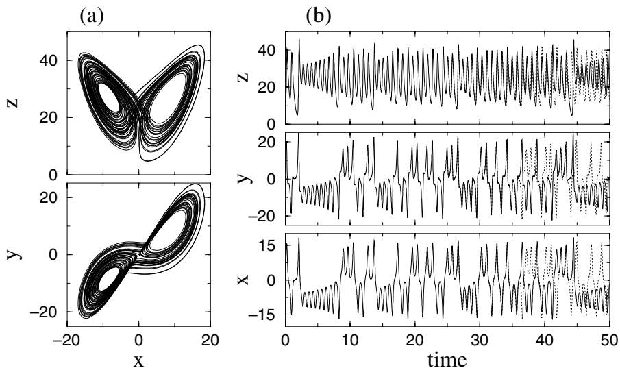
Figure 5.2. The dynamics of the Lorenz system (see Eqs. (10.4)). (a) Projections of the phase portrait on planes (x, y) and (x, z) . Note the symmetry x \rightarrow -x , y \rightarrow -y . (b) The time series of the variables x , y , z (solid curves). In this figure we also demonstrate the sensitivity to small perturbations: at time t = 25 a perturbation 10^{-4} is added to the x variable. The perturbed evolution, shown with the dashed curve, very soon diverges from the original one and demonstrates a different pattern of oscillations.
