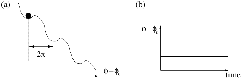
Figure 3.5. Small detuning. The external force creates minima in the tilted potential (a) and the particle rests in one of them. This corresponds to a stable constant phase difference, \phi - \phi_e = \phi^0 + \Delta\phi (b).
