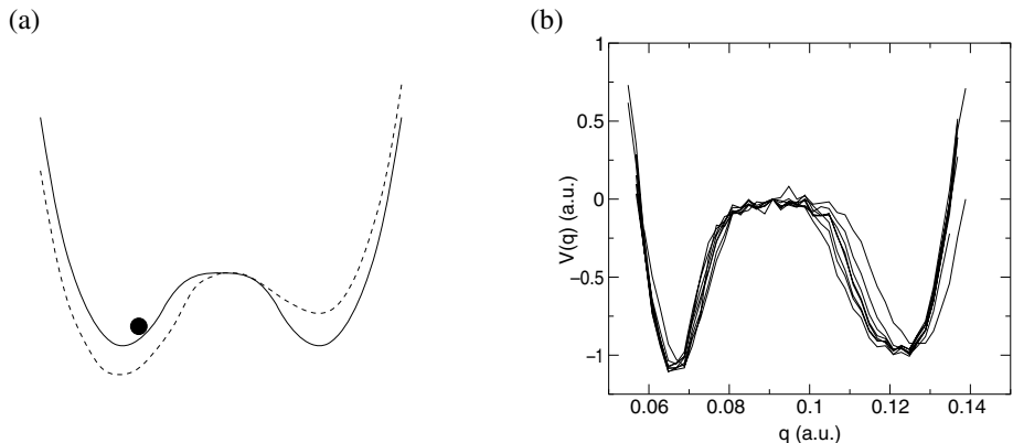
Figure 3.49. (a) Motion of a particle in a double-well potential. Noise induces irregular transitions between two stable states. A weak periodic force acting on the system modifies the potential so that the height of the wells is varied periodically (one snapshot is shown by a dashed line). (b) The effective bistable potential V(q) obtained from the data of a laser experiment (the spatial coordinate and the potential height are in arbitrary units). Part (b) from Barbay et al. , Physical Review E , Vol. 61, 2000, pp. 157–166. Copyright 2000 by the American Physical Society.
