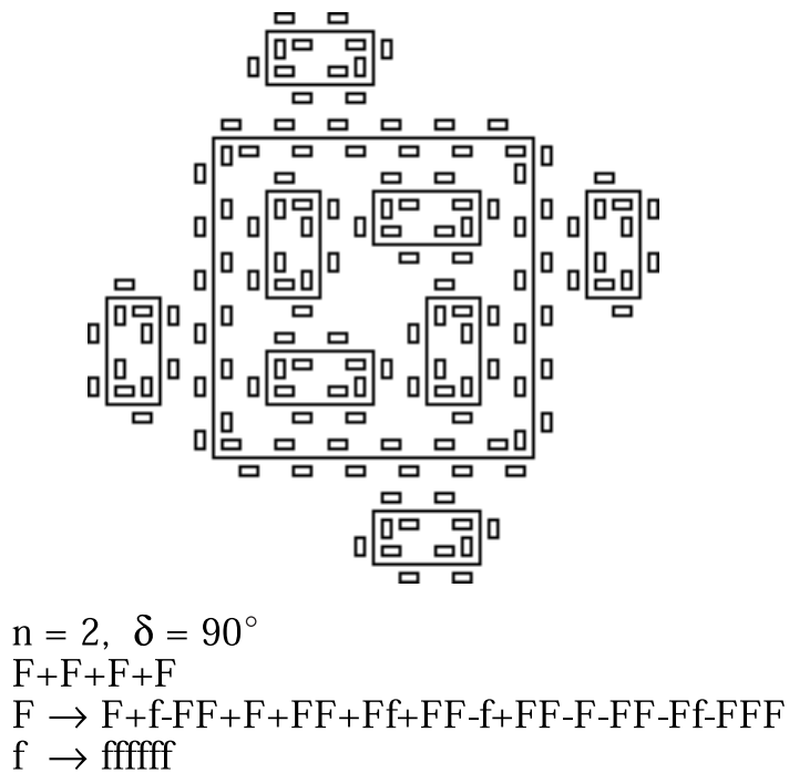
Figure 1.8: Combination of islands and lakes [95, page 121]
