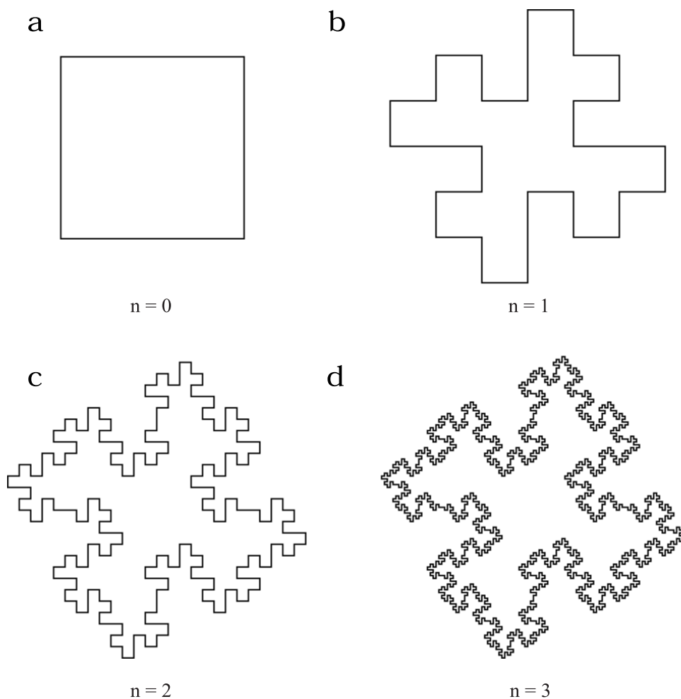
Figure 1.6: Generating a quadratic Koch island
