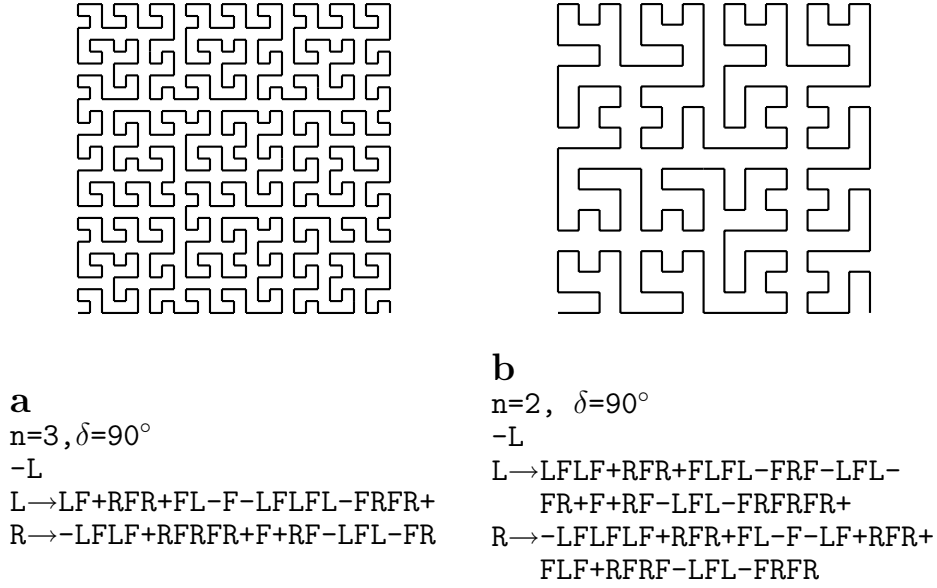
Figure 1.16: Sample FASS curves constructed using tiles with contact points positioned along a tile edge: (a) 3 \times 3 tiles form a macrotile, (b) 4 \times 4 tiles form a macrotile
