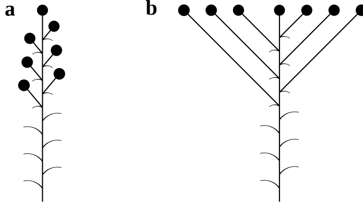
Figure 3.7: Closed racemes: (a) elongated form, (b) planar form
