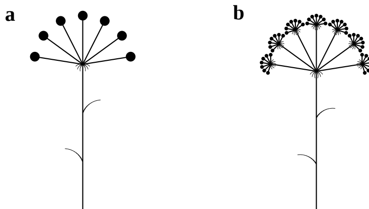
Figure 3.22: Umbels: (a) simple, (b) compound
