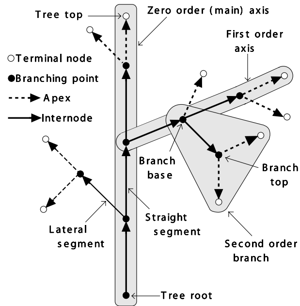
Figure 1.20: An axial tree
