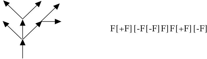
Figure 1.23: Bracketed string representation of an axial tree
