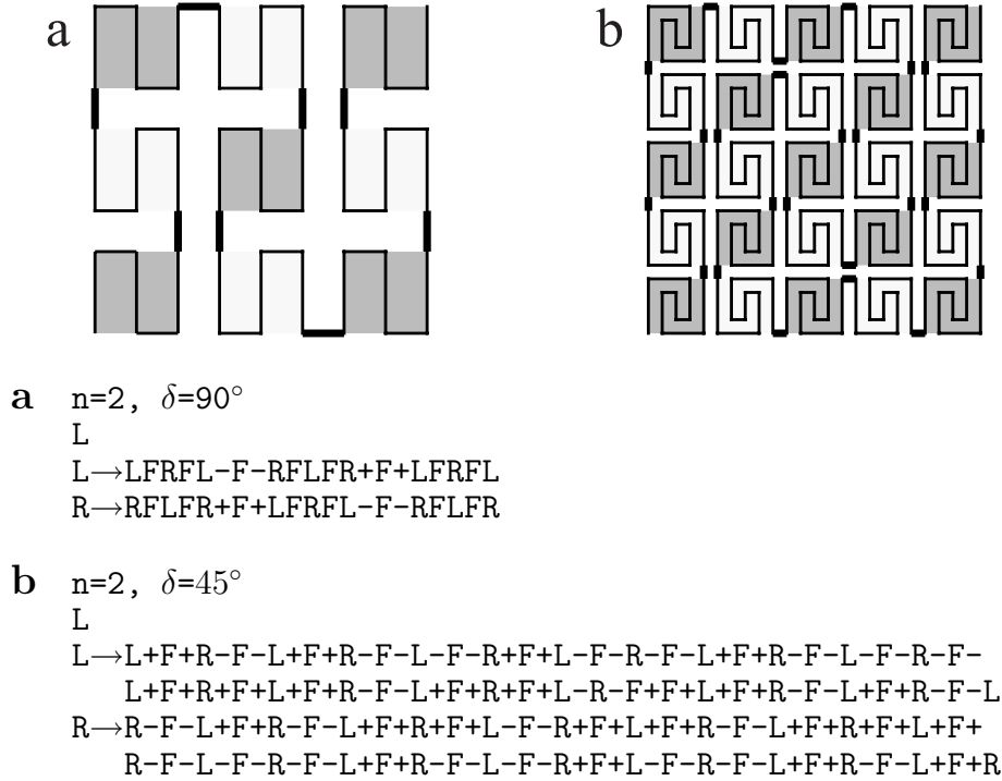
Figure 1.17: Sample FASS curves constructed using tiles with contact points positioned diagonally: (a) 3 \times 3 tiles form a macrotile (Peano curve [106]), (b) 5 \times 5 tiles form a macrotile
