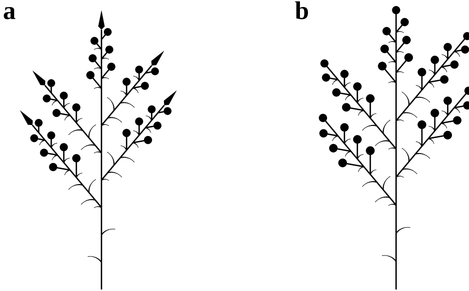
Figure 3.8: Dibotryoids: (a) open, (b) closed
