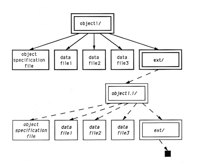
Figure A.1: The hierarchical structure of objects
