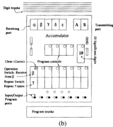
Figure 11 (a) View of an Accumulator's front panel. The operation switch's settings are a, b, g, d, e , O, A, S and AS. The repeat switch's settings are 1 through 9. (b) Simplified front panel.
