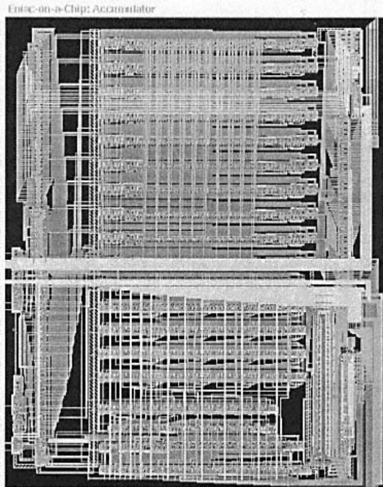
Figure 26 Layout of one of the twenty Accumulators. The size is 550\text{ }\mu\text{m} \times 800\text{ }\mu\text{m} . Floor Plan and Layout of an Accumulator.
