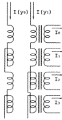
Figure 8 Word selector
