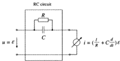
Figure 24 Phase modifier
