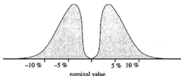
Figure 3 Distribution of \pm 10\% Resistor Values
