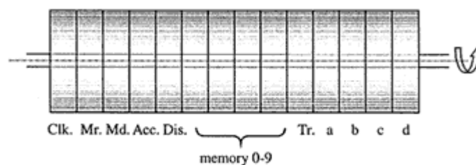
Figure G1 memory drum
