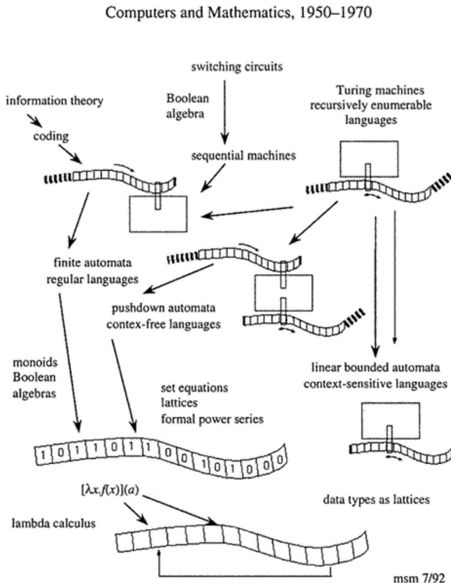
Figure 2 Machines and Languages
